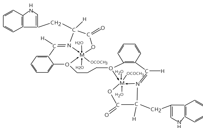
Figure 1. The proposed structure for the metal complex compound ( M = \text{Zn} ).
